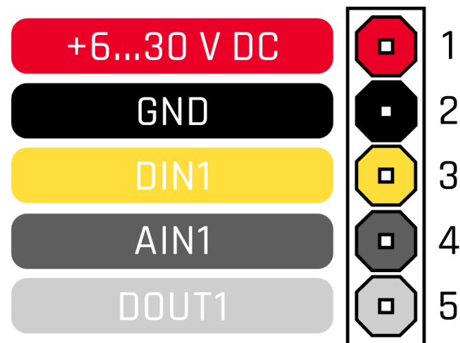
Figure 2 FMB900 pinout
